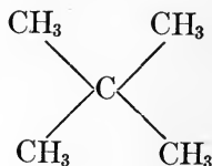
Tetramethyl-methane
